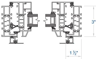
SECTION B-B: JAMBS
