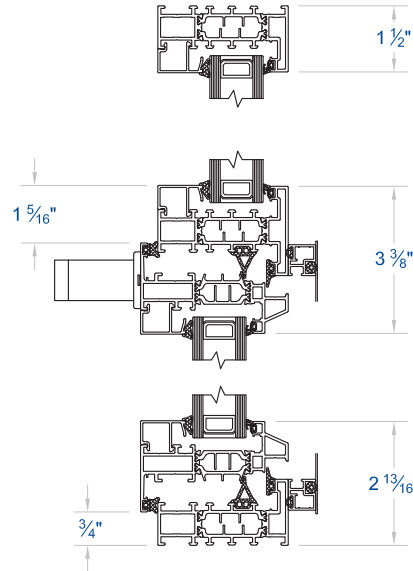
SECTION C-C: HEAD / SILL
